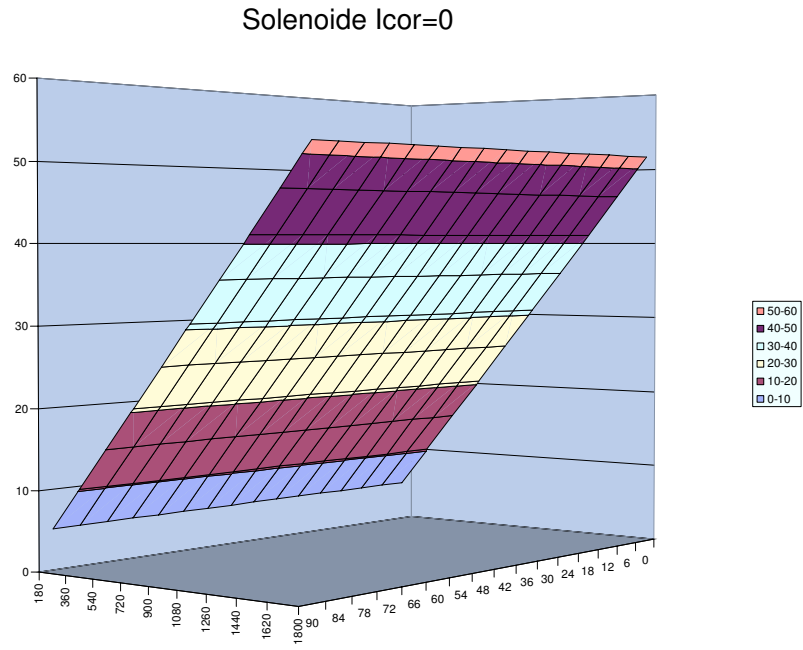
Figure 1: Configuration 1 for the coil: no correction coils, no anti-DID \int_{\ell_{\text{drift}}} \frac{B_r}{B_z} dz \simeq 54\text{mm max.}
