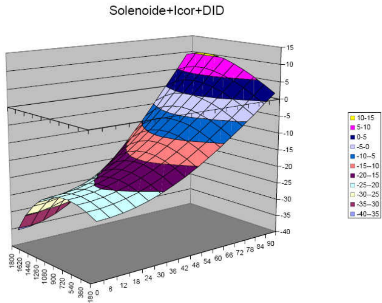
Figure 4: Configuration 4, add anti-DID \int_{\ell_{\text{drift}}} \frac{B_x}{B_z} dz \simeq 35\text{mm} max.
