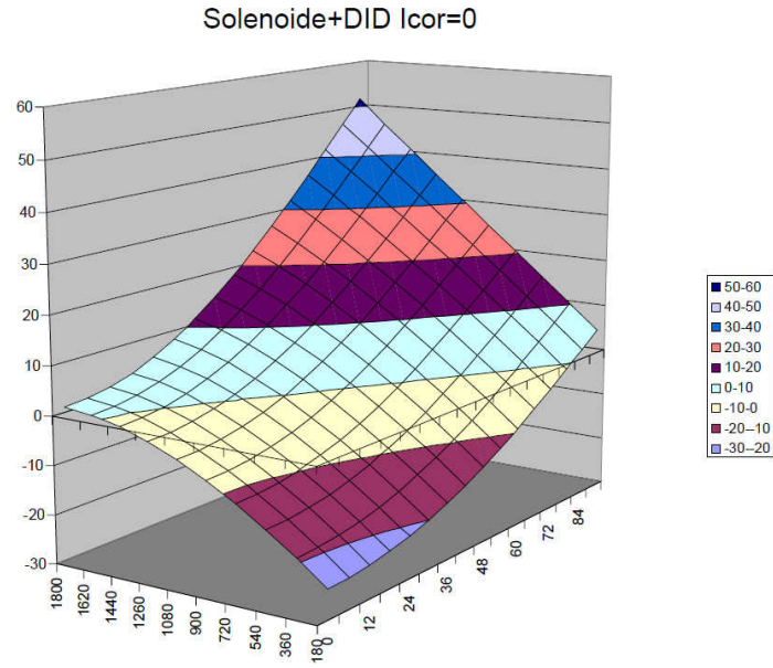
Figure 3: Configuration 3, no correction coils and with anti-DID \int_{\ell_{\text{drift}}} \frac{B_x}{B_z} dz \simeq 50\text{mm} max.
